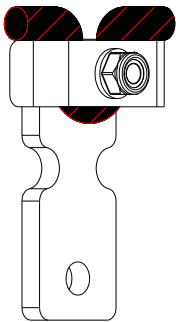
REAR ISO VIEW FOR INTERMEDIARY MASTER RUNNER
