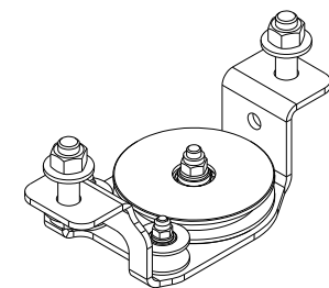
TRA1001
